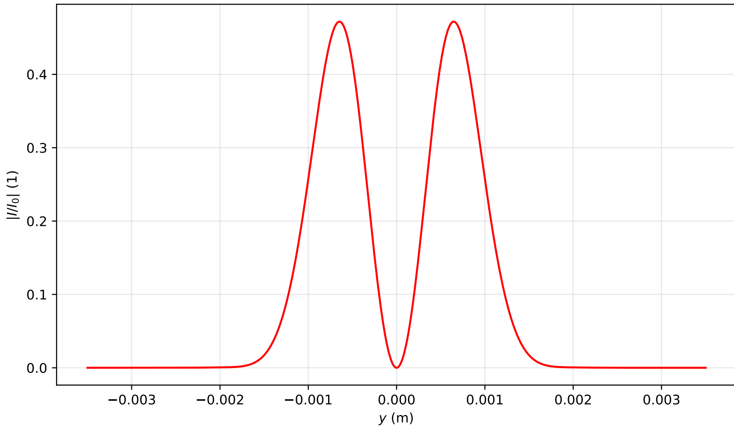
Intensity profile I(x=0, y, z=1.672)/I_0 , P_{in}=1.0P_{cr} , artificial time
